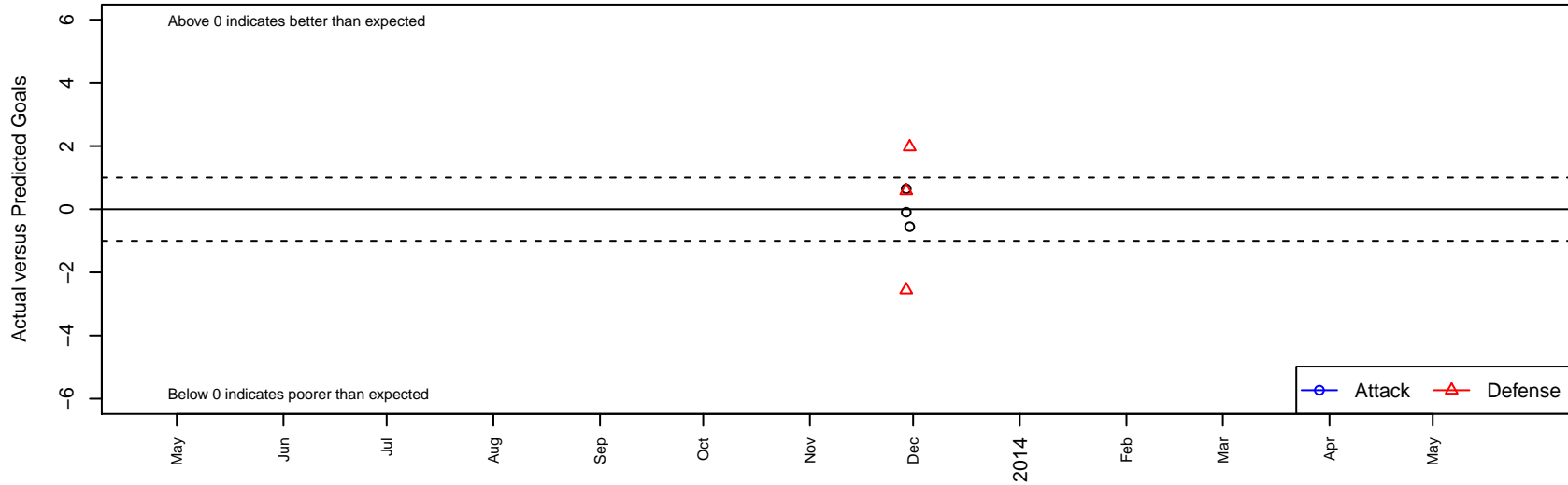
Celtic Hoops G02 Dots are actual minus expected GF (blue circles) and GA (red triangles). Blue line is smoothed change in attack strength. Red is smoothed change in defense strength.
